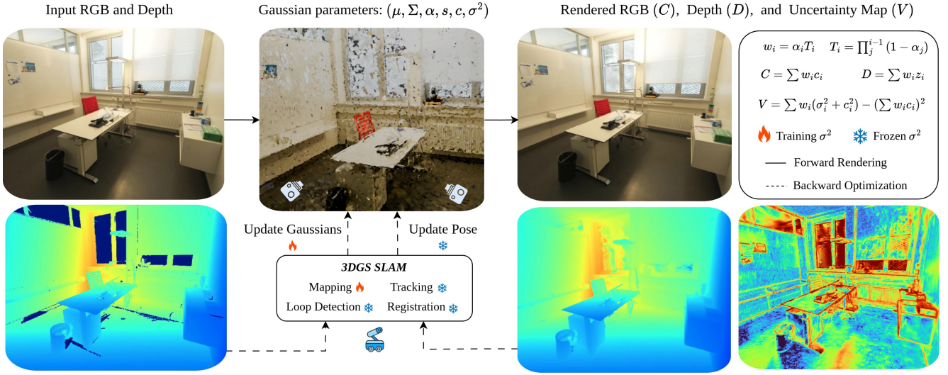
Figure 1. VarSplat. Given RGB-D inputs, each 3D Gaussian jointly learns position, orientation, scale, color, opacity, and appearance variance \sigma^2 . During mapping, \sigma^2 is optimized jointly with other Gaussian parameters. The rendered per-pixel uncertainty V serves as a confidence weight during tracking and registration, while the per-Gaussian variance \sigma^2 further guides loop detection, enabling robust and uncertainty-aware SLAM.
